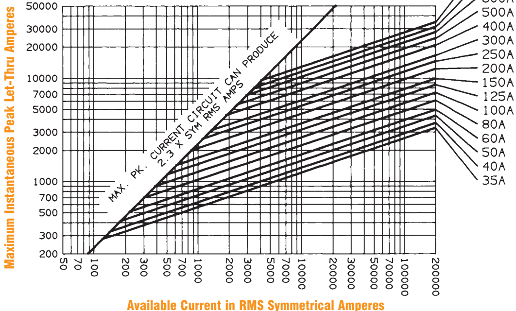
Peak Let-Through Current Data – A70QS35 to 800, 700 Volts AC
